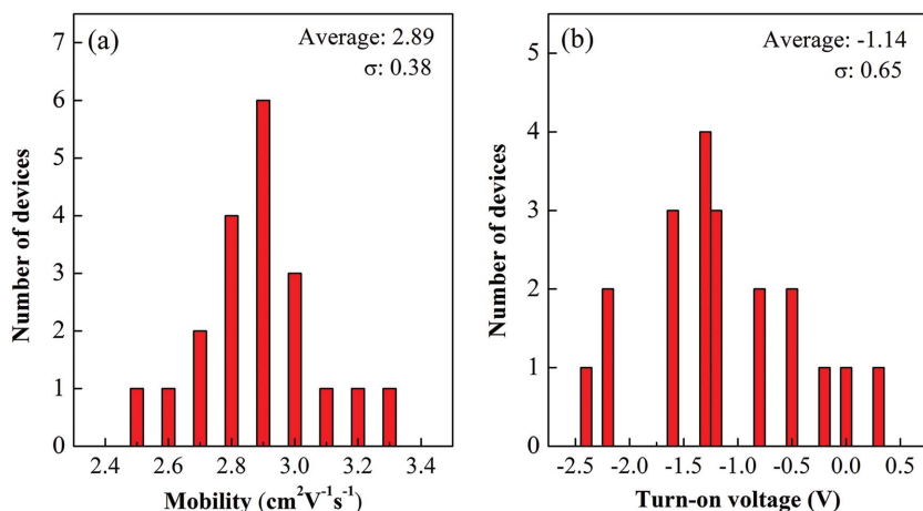
Figure 5. Histogram of the a) mobility and b) turn-on voltage for IZO TFTs ( 4 \times 5 array) processed at 230 °C for 4 h. \sigma represents the standard deviation.
